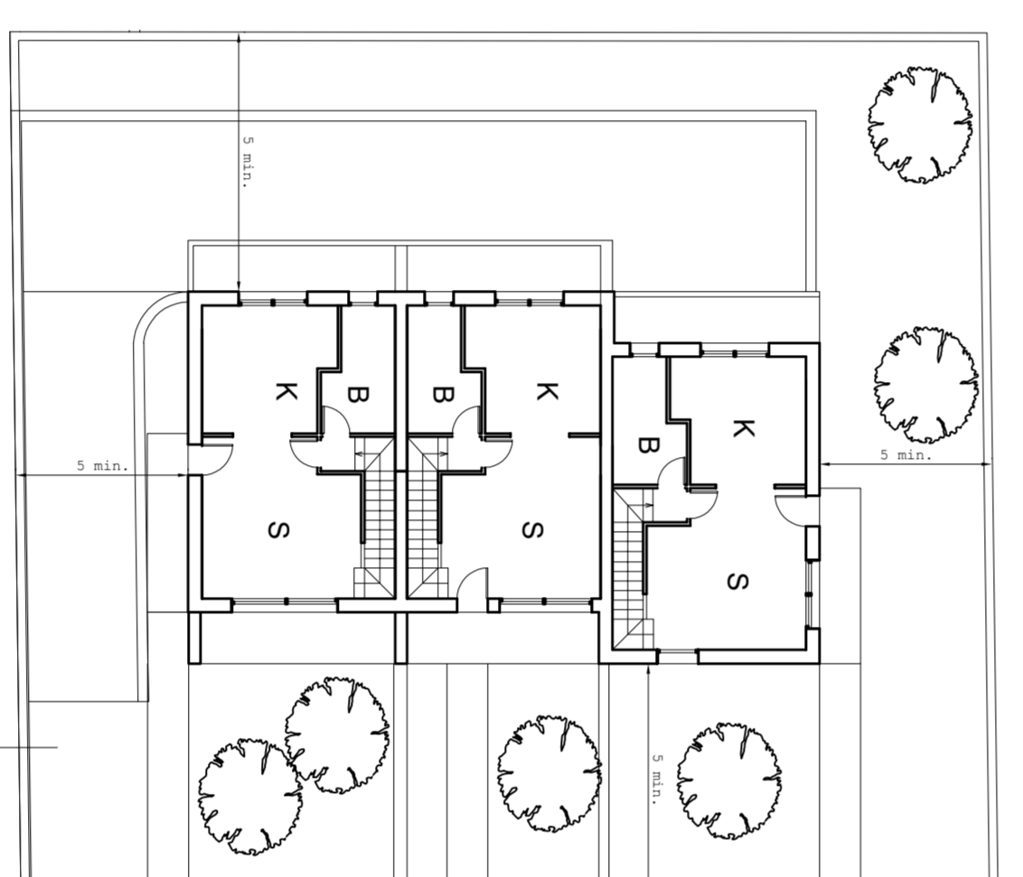
PIANO TERRA
