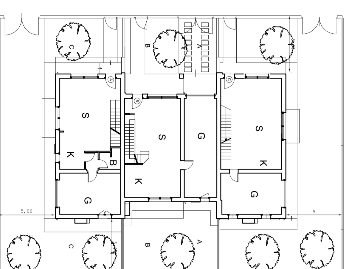
PIANO TERRA
